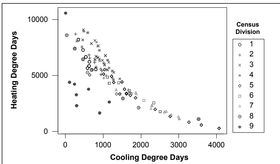
Figure 1. Heating Degree Days vs. Cooling Degree Days for CBECS Offices
